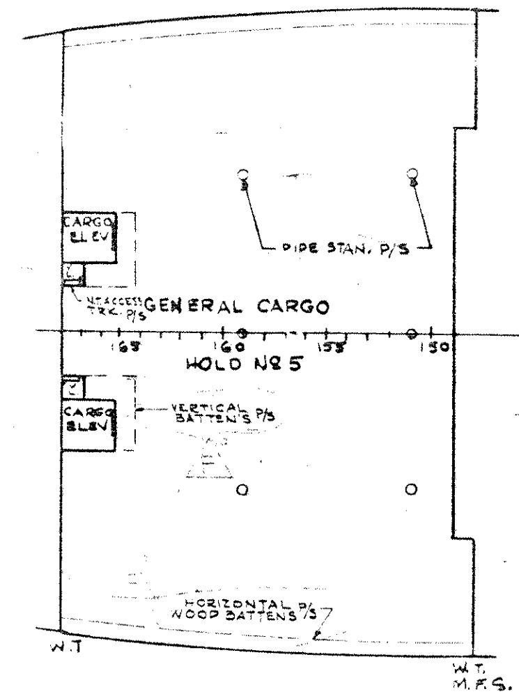
24'-6" FLAT
