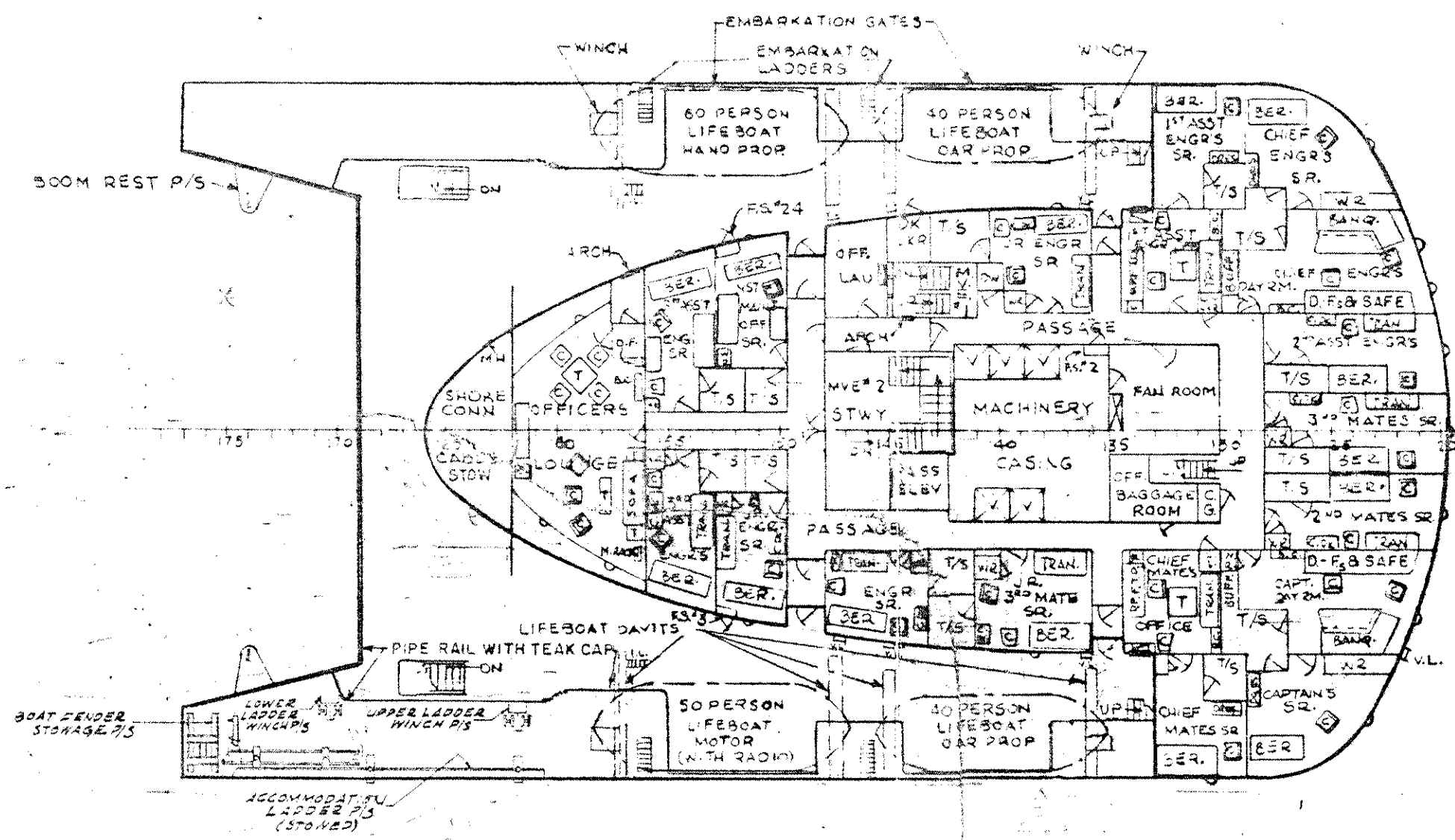
BOAT DECK
